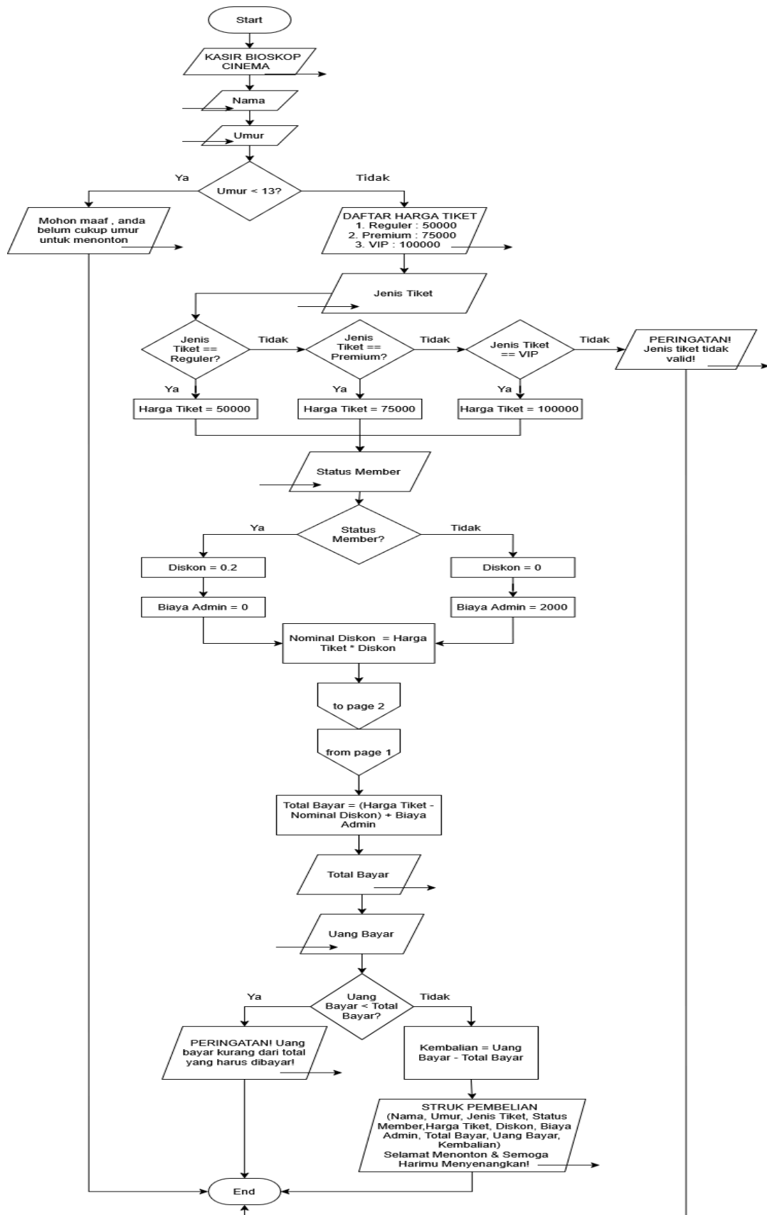
Gambar 1.1. Flowchart Kasir Bioskop Cinema
